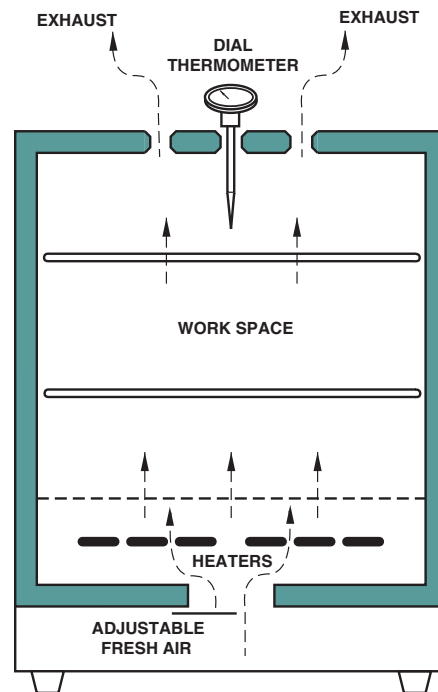
Circulation Diagram (Front View)
