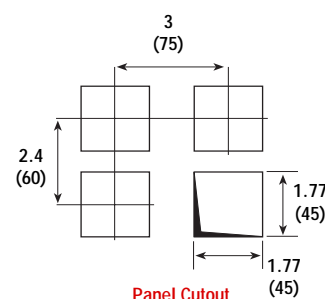
Panel Cutout
